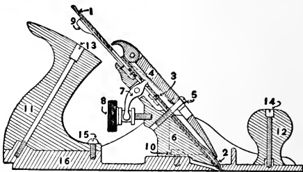
Fig. 10—Section of Plane
